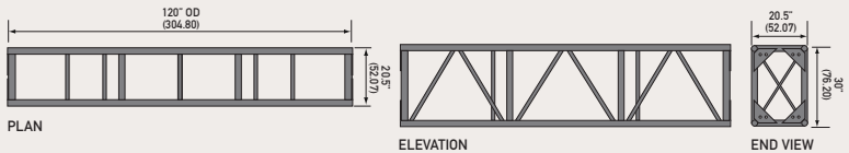
PLAN VIEWS
