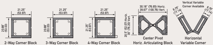
PLAN VIEWS
